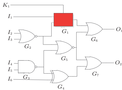
Fig.7. Gate-level netlist with a binding cell.
