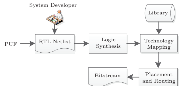
Fig.2. Typical FPGA design flow with the new binding from RTL to layout.
