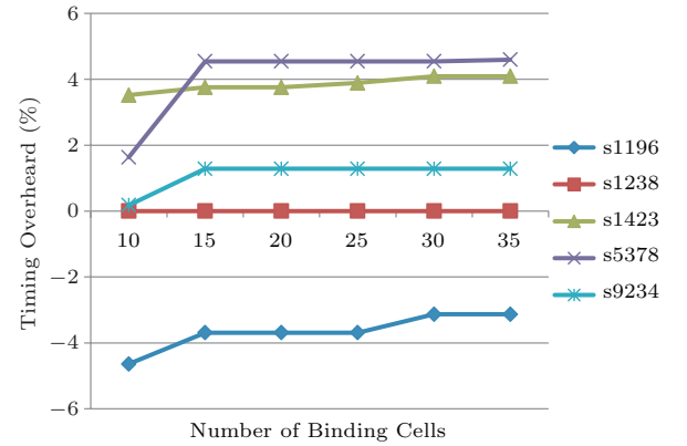
Fig.9. Timing overhead trend on benchmark circuits with different numbers of binding cells.
