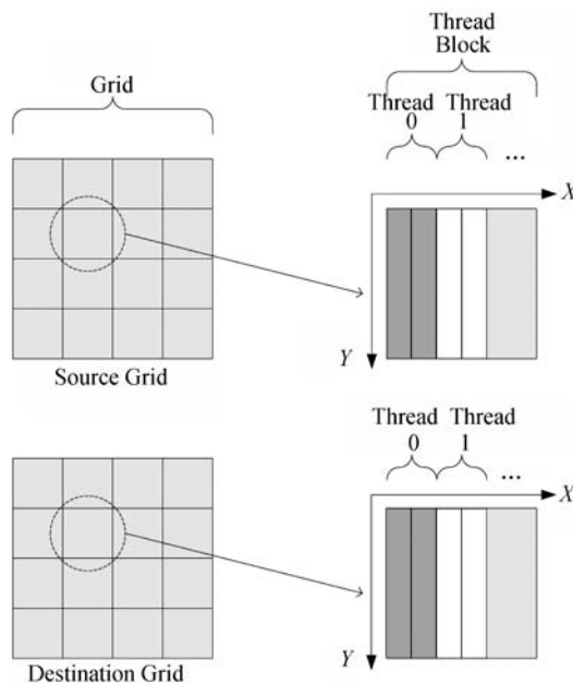
Fig.1. Decomposition of 2D grids. Source and destination grids are divided into tiles, each of which is handled by a thread block. Within each thread block, threads are organized in 1D. Each thread is in charge of a few consecutive points in the X-direction, and computes all the way through the Y-direction.
