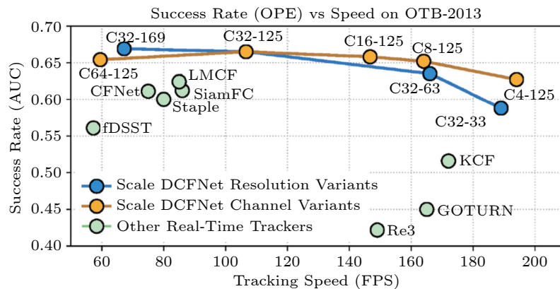
Fig.5. Tracking speed and AUC performance on OTB-2013 [54] . The tracking speed ranges from 60 FPS to 190 FPS with different input spatial resolutions and different numbers of the output feature channels. “CX-Y” stands for a member in the scale DCFNet family consisting of X output feature channels and Y×Y input resolution. For example, “C32-169” means that our scale DCFNet has 32 channels and 169×169 resolution.
