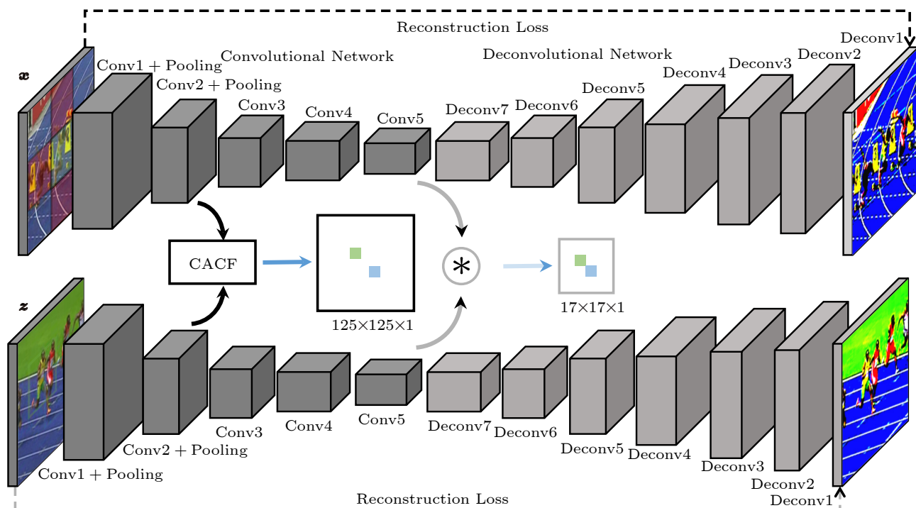
Fig.4. Architecture of our convolutional-deconvolutional DCFNet. The “ 125 \times 125 \times 1 ” is the size of a correlation response map from CACF. The “ 17 \times 17 \times 1 ” is the size of a correlation response map from the high-level semantic correlation analysis. Conv i : the i -th convolutional layer, Deconv j : the j -th devolutional layer.
