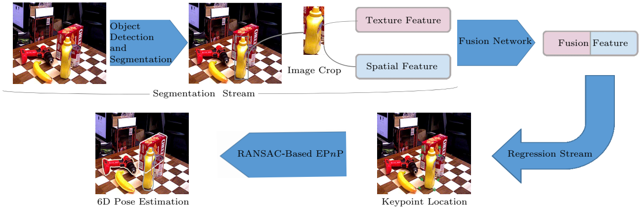
Fig.2. Proposed network architecture. A two-stream architecture network is designed for feature processing, including segmentation and regression. A fusion network that can combine texture and spatial features also exists.
