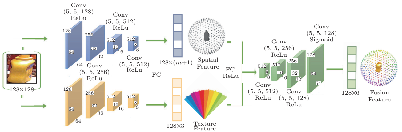
Fig.4. Architecture of the fusion network. This detailed flowchart explains the process of extracting spatial and texture information on the basis of heterogeneous CNN, and then feeds them into another one to obtain fusion features. m+1 refers to the (m+1) -channelled semantic segmentation map in Subsection 3.2 and 6 includes XYZ and RGB.
