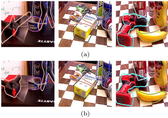
Fig.9. Comparison of the iterative refinement module. (a) Original estimation of the main network. (b) Results presenting the benefits of our end-to-end procedure for large occlusions.
