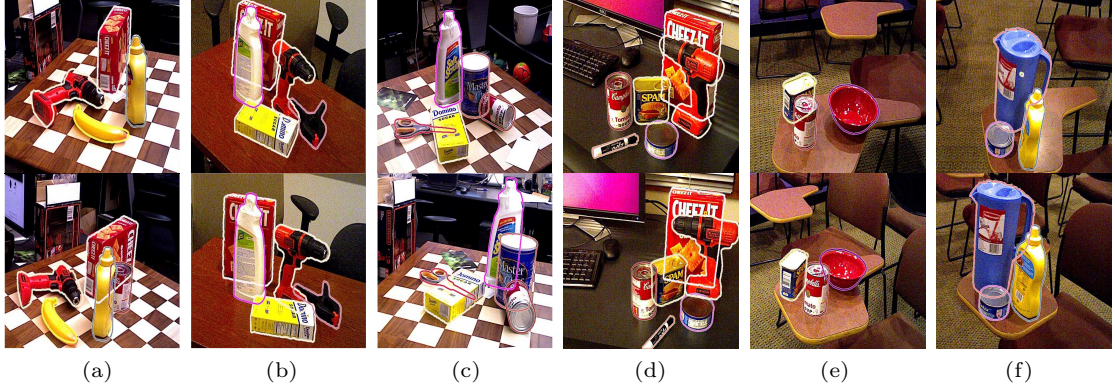
Fig.8. YCB-Video results. (a)–(f) Each pair of images represents different perspectives of the same scene. Our method generates accurate pose estimations, even in the presence of large occlusions. Furthermore, it can process multiple objects in real time.
