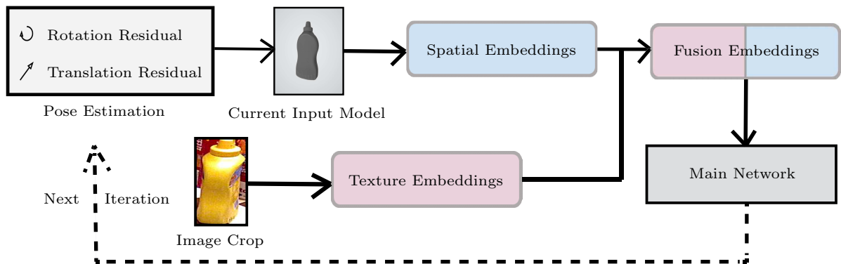
Fig.3. Refinement procedure with the end-to-end mechanism. This additional iterative optimization directly follows the main network.
